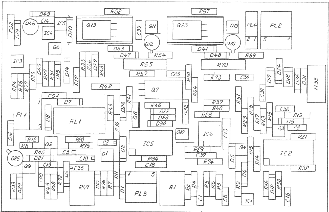
PCB ASSEMBLY DRAWING 622 VERSION 2A
