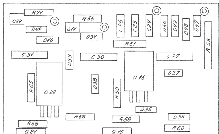
PCB ASSEMBLY DRAWING 623 VERSION 1A
