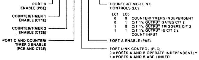
Figure B-1. Master Control Registers
