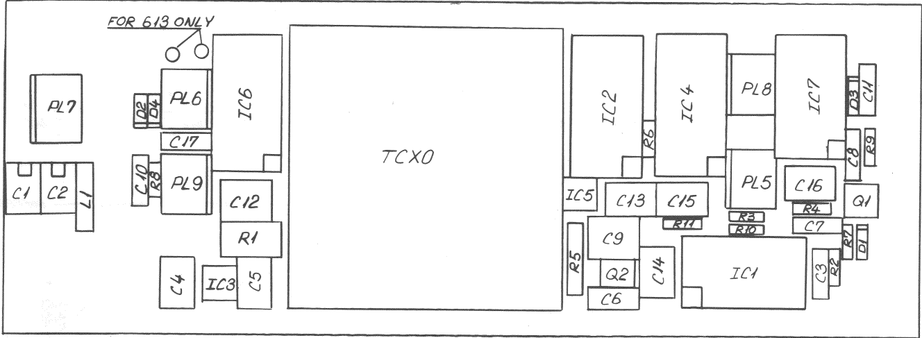
PCB ASSEMBLY DRAWING 612 613 614 VERSION 2A
