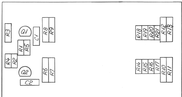
PCB ASSEMBLY DRAWING 699 VERSION 1A
